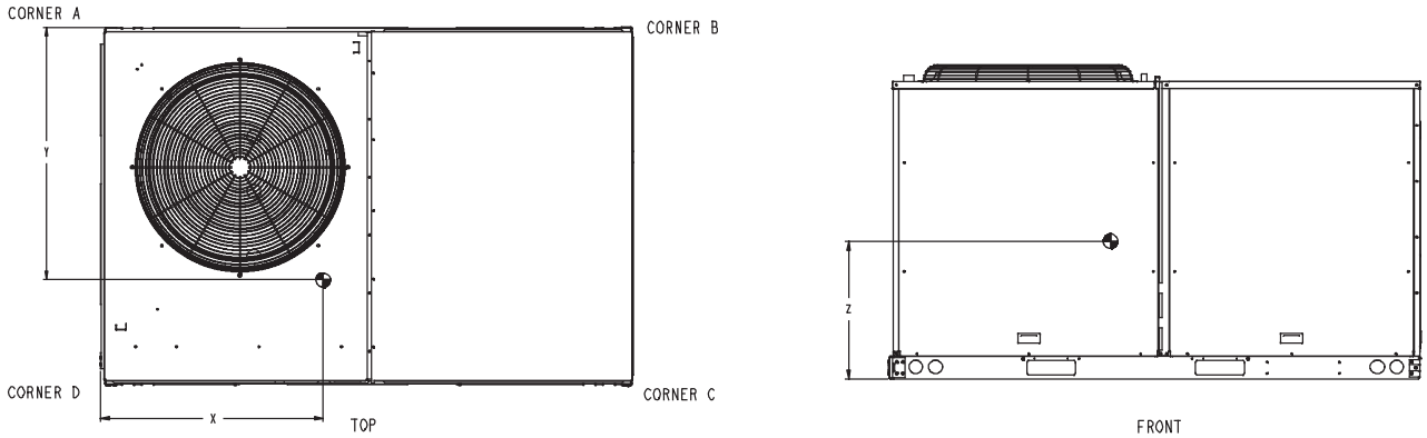
Dimensions 50TCMD 09/12/13
